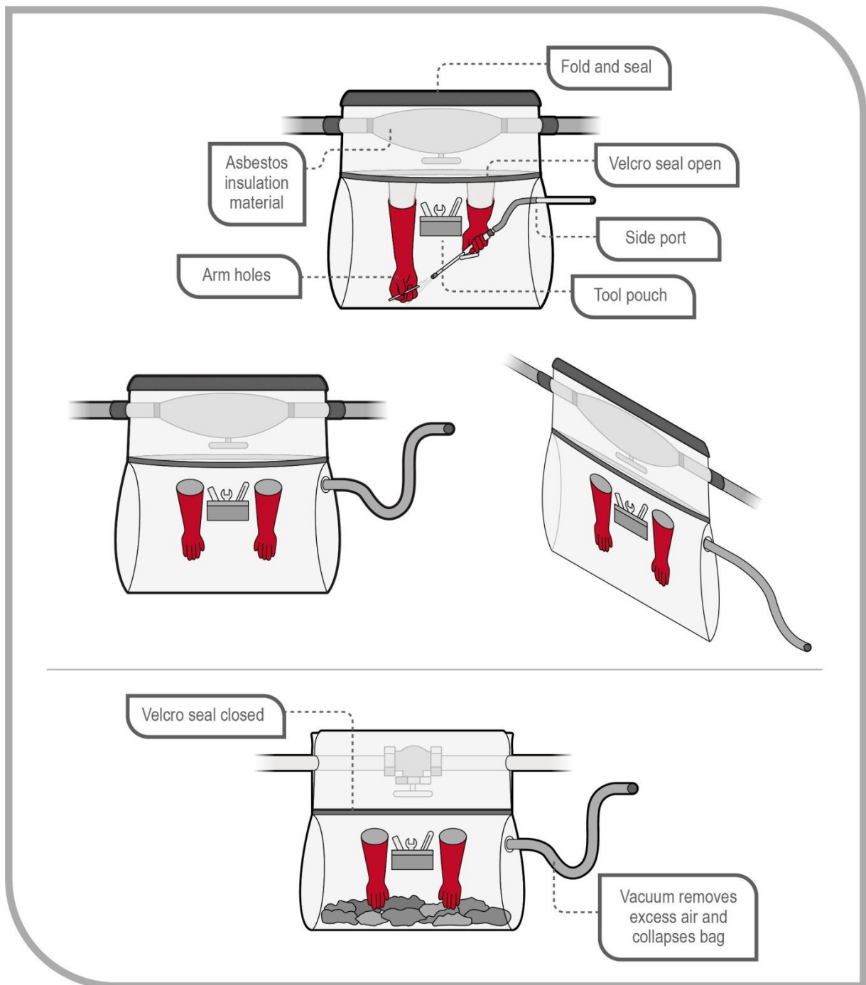
Figure 9: Example of a glove bag
