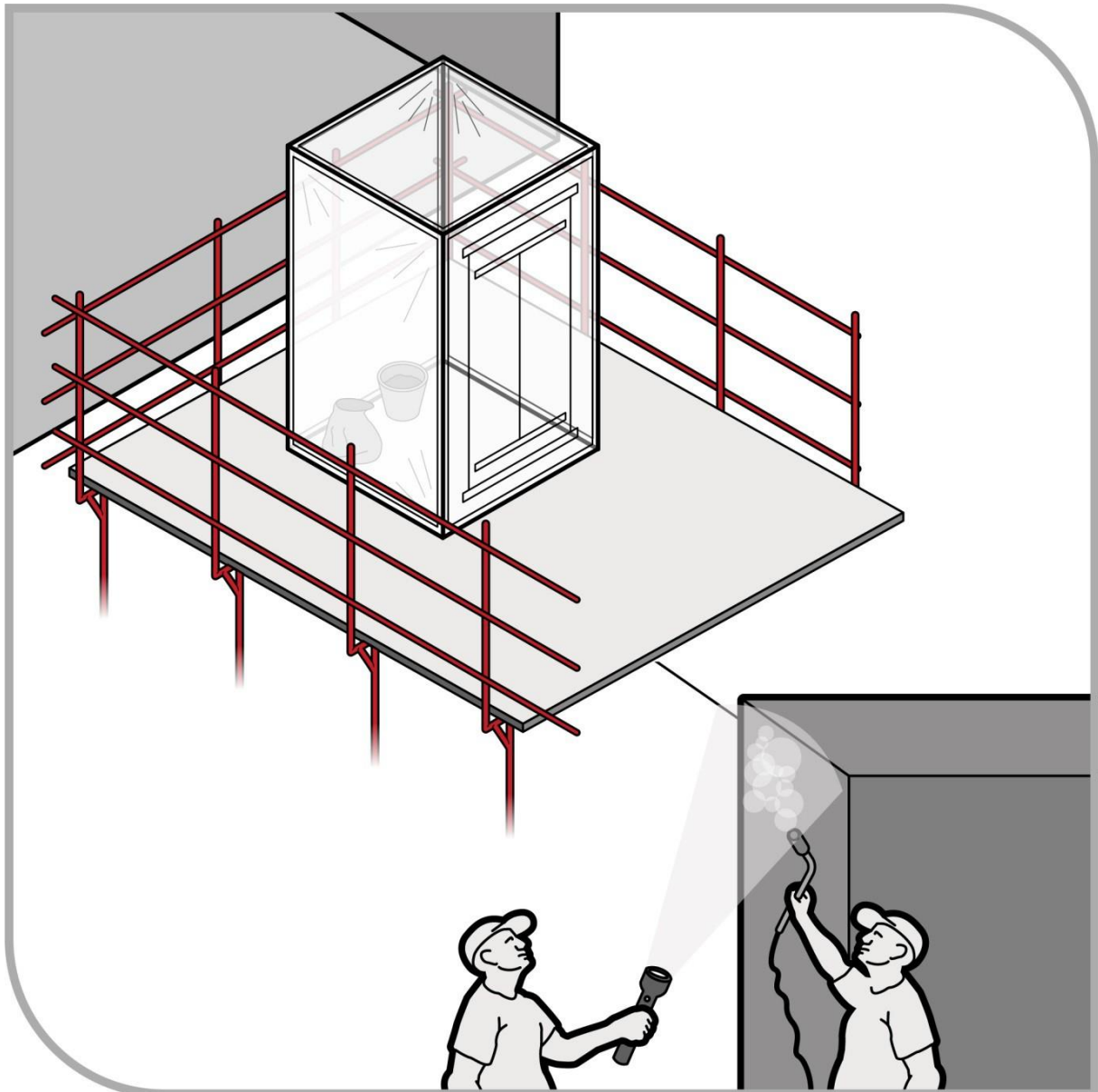
Figure 8: Building and using the enclosure
