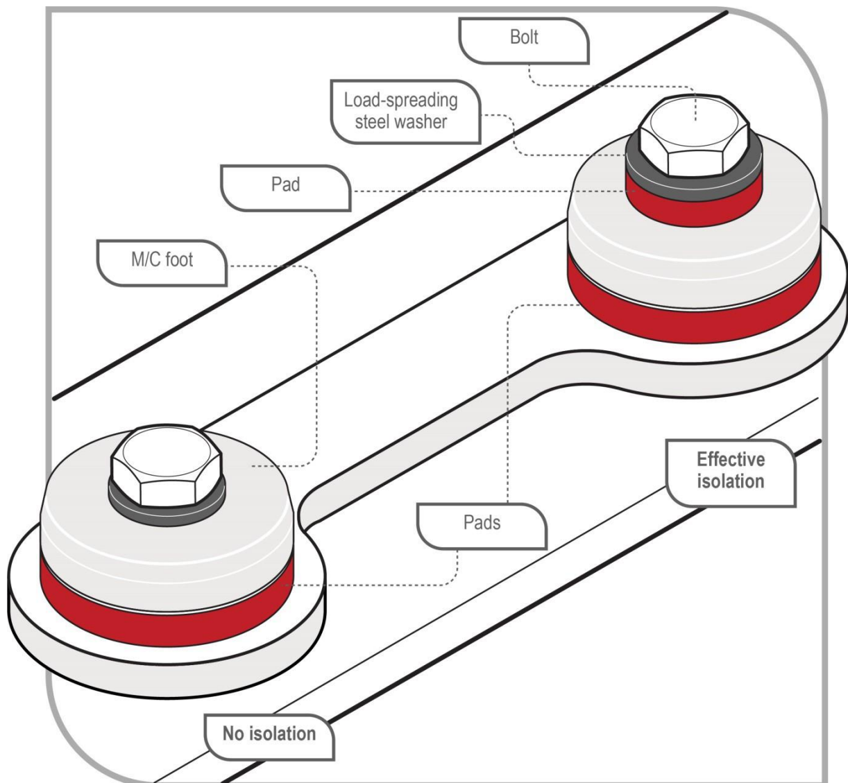
Figure 8 Image demonstrating effective and ineffective isolation
