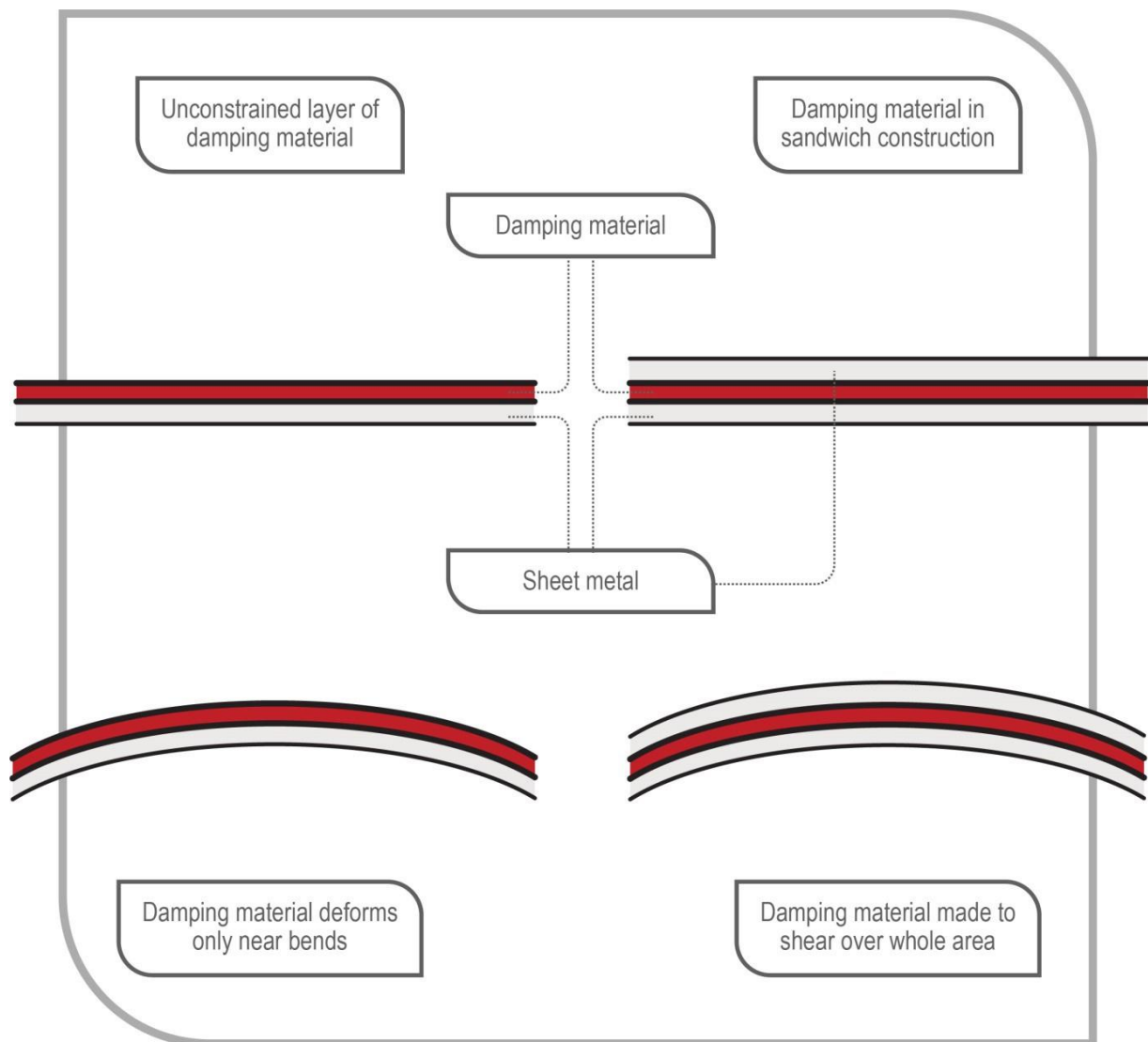
Figure 4 Damping
